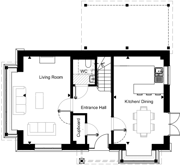
Plot 01 Ground Floor Living Room 3113mm x 5763mm / 10'-3" x 18'-11" Kitchen/ Dining 3313mm x 5785mm / 10'-10" x 19'-0"
