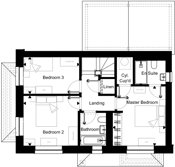
Plot 01 First Floor Master Bedroom 3446mm x 3870mm / 11'-4" x 12'-8" Bedroom 2 3654mm x 3256mm / 12'-0" x 10'-8" Bedroom 3 3654mm x 2395mm / 12'-0" x 7'-10"
